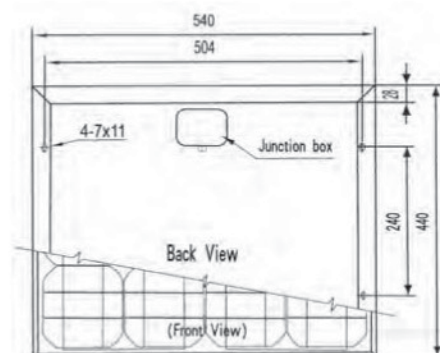
Blueprint of the module
